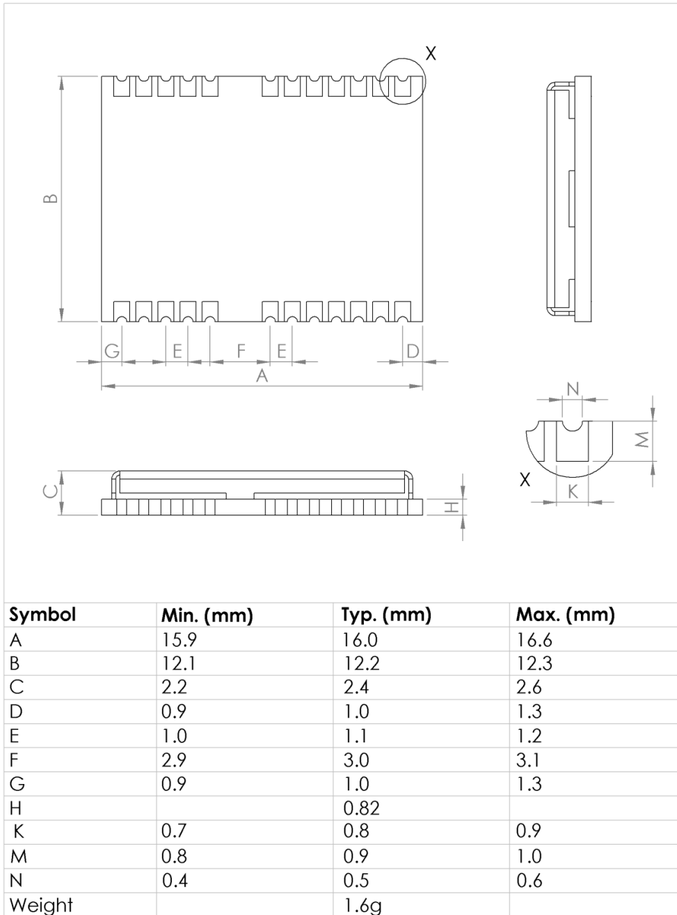
Figure 4: Dimensions
