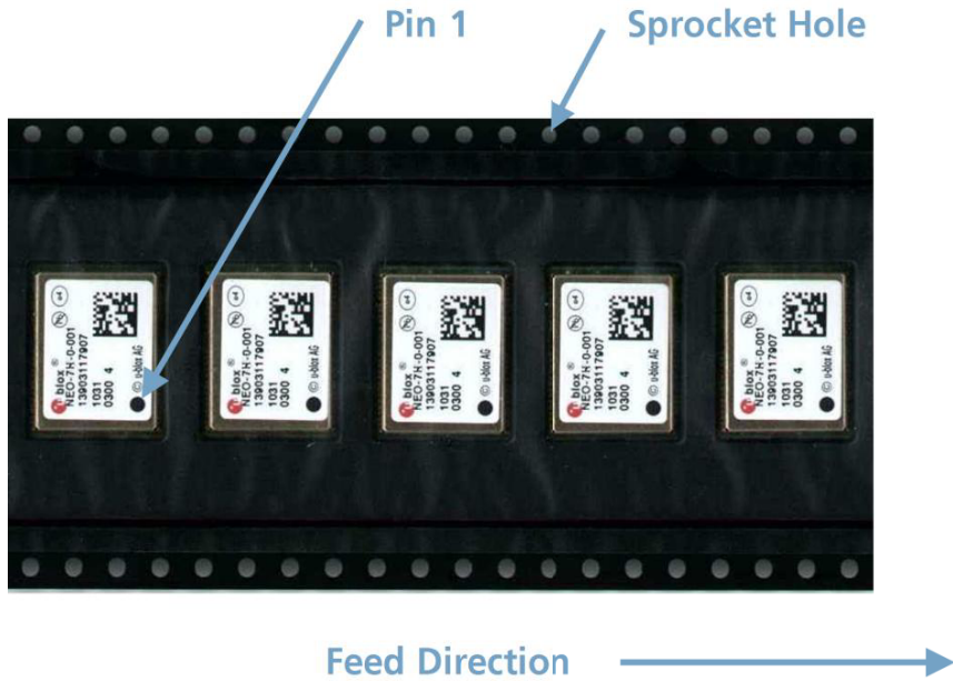
Figure 6: Orientation for NEO-6 modules on tape
