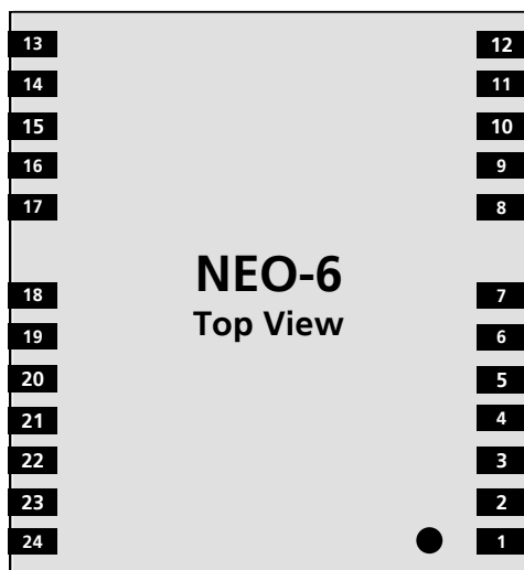
Figure 2 Pin Assignment
